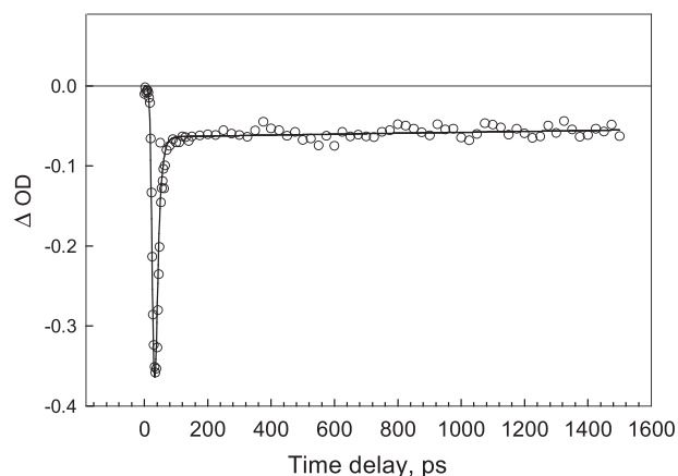
Figure 4. Transient absorption decay for \text{Co}^{\text{II}}\text{TMpyP}(4) in \text{poly}(\text{dA-dT})_2 with excitation at 540 nm and probe at 425 nm. Solid line curve represents a least-square fit to a double-exponential function. Fitted decay times are: 10 \pm 3 ps (fast component) and 10 \pm 4 ns (slow component).
