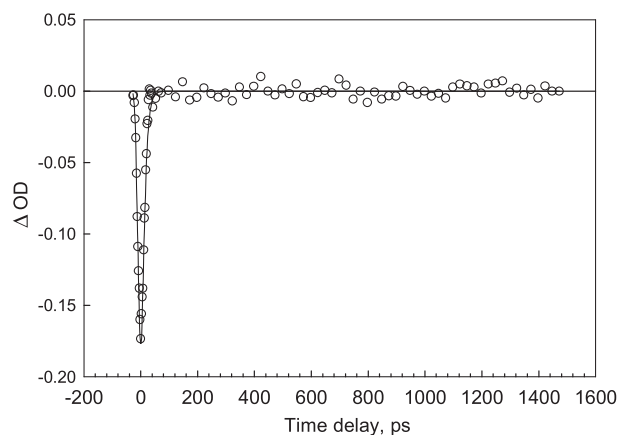
Figure 3. Transient absorption decay of \text{Co}^{\text{III}}\text{TMpyP}(4) - DNA complex with excitation at 540 nm and probe at 434 nm. Solid line curve represents a least-square fit to a single-exponential function with 10 \pm 3 ps time constant.
